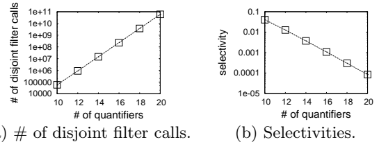
Figure 3: Disjoint filter selectivity tests for star queries by varying the number of quantifiers.
