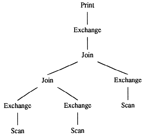
Fig. 5. Operator model of parallelization.
