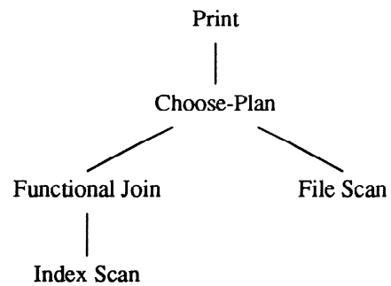
Fig. 4. A dynamic query evaluation plan.
