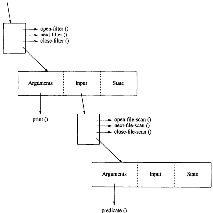
Fig. 2. Two operators in a query evaluation plan.
